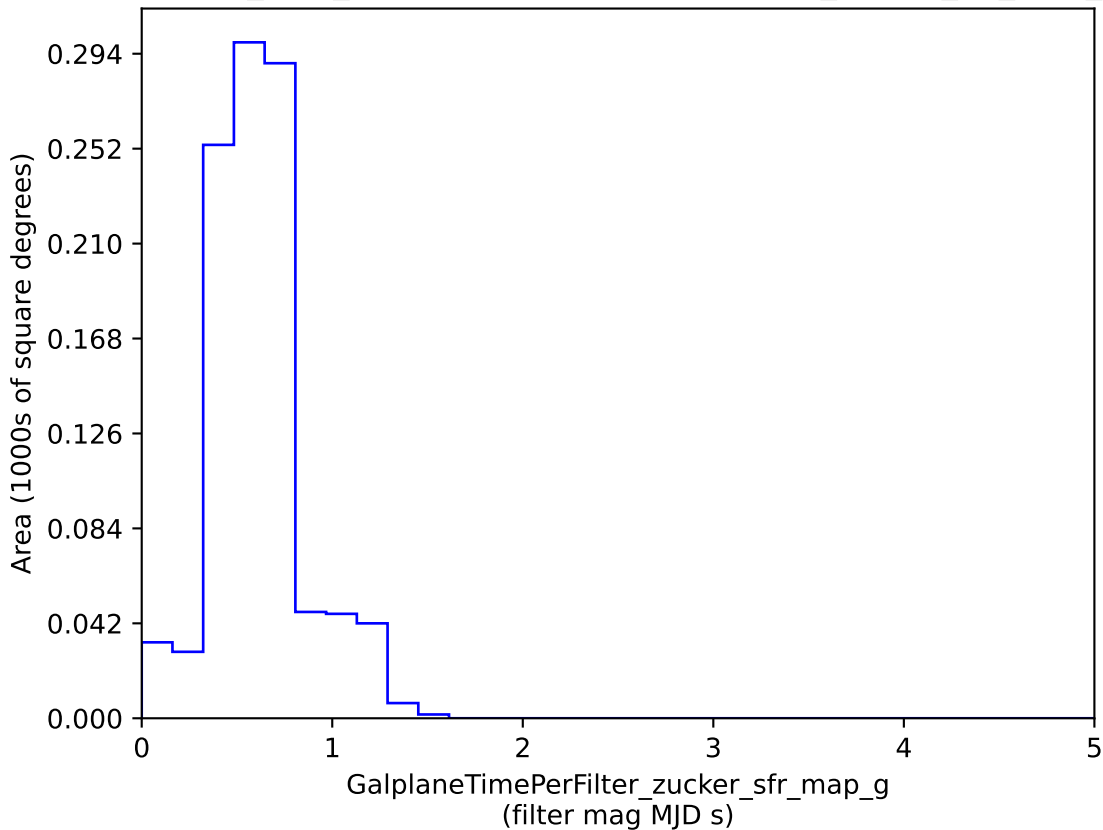
baseline_v3.2_10yrs : GalplaneTimePerFilter_zucker_sfr_map_g
