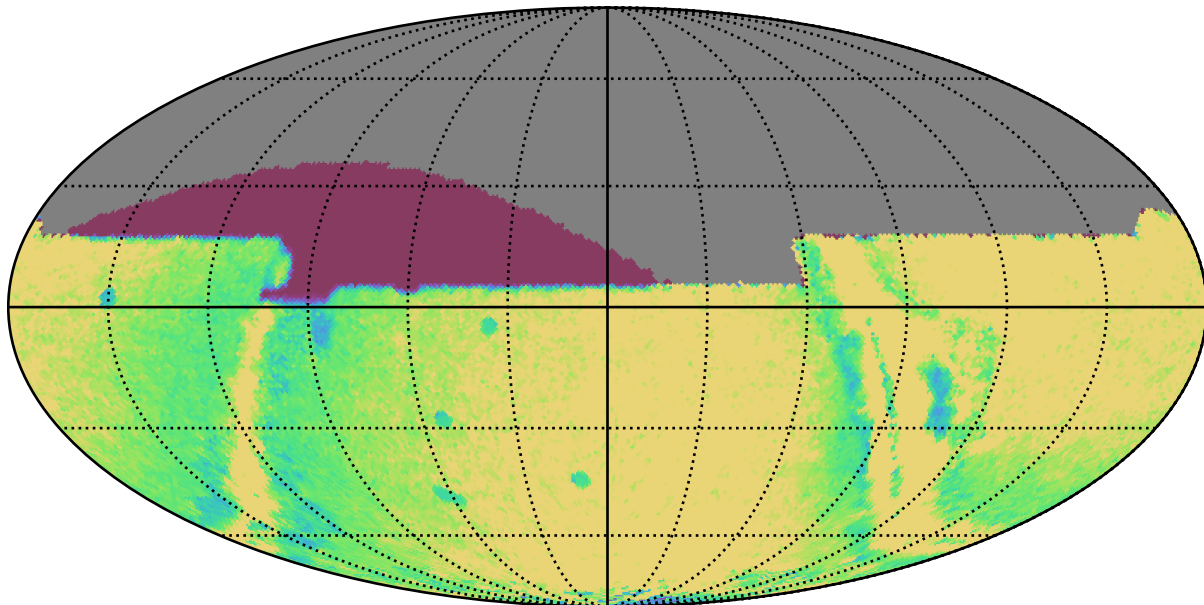
baseline_v3.2_10yrs : GalplaneTimePerFilter_xray_binaries_map_y
