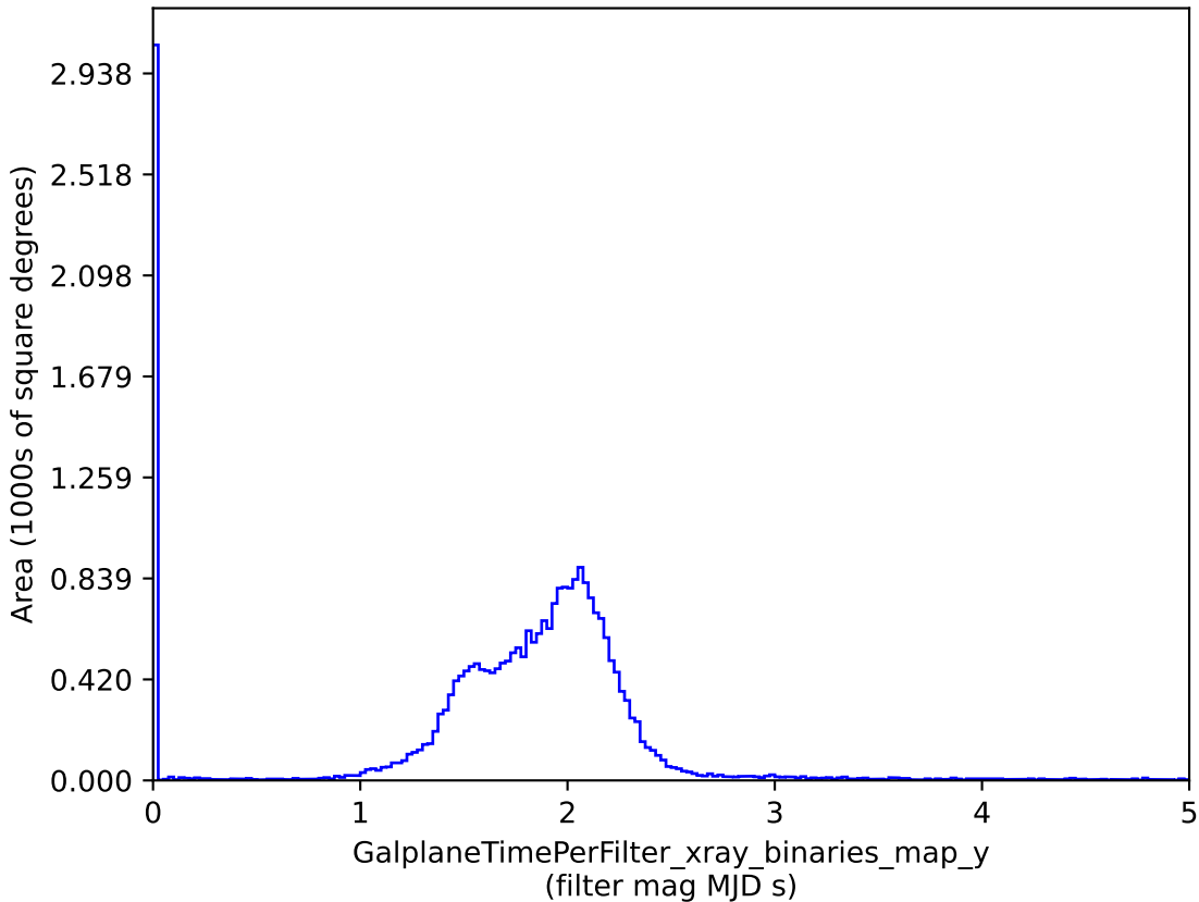
baseline_v3.2_10yrs : GalplaneTimePerFilter_xray_binaries_map_y
