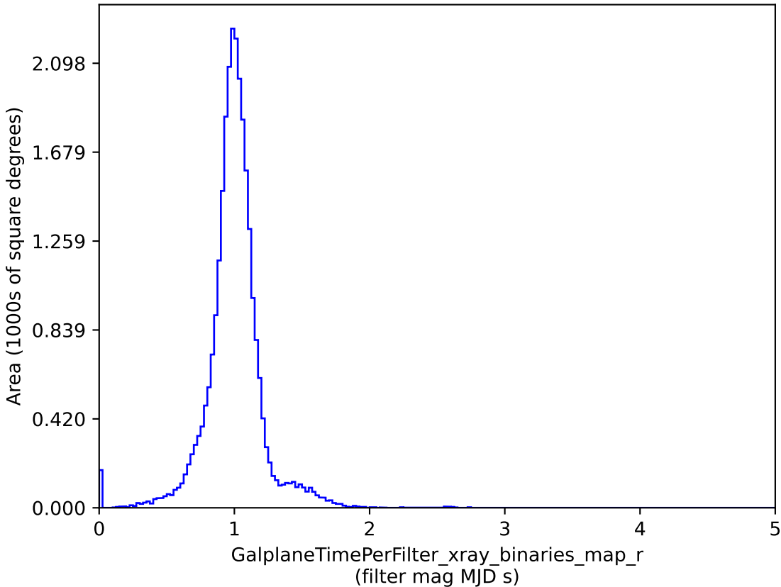
baseline_v3.2_10yrs : GalplaneTimePerFilter_xray_binaries_map_r
