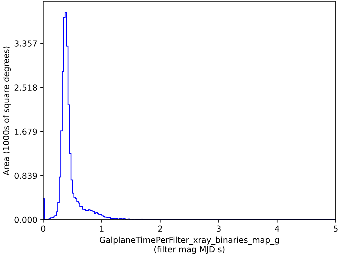
baseline_v3.2_10yrs : GalplaneTimePerFilter_xray_binaries_map_g
