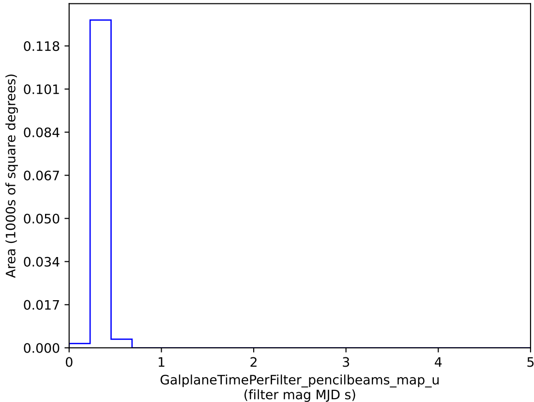
baseline_v3.2_10yrs : GalplaneTimePerFilter_pencilbeams_map_u
