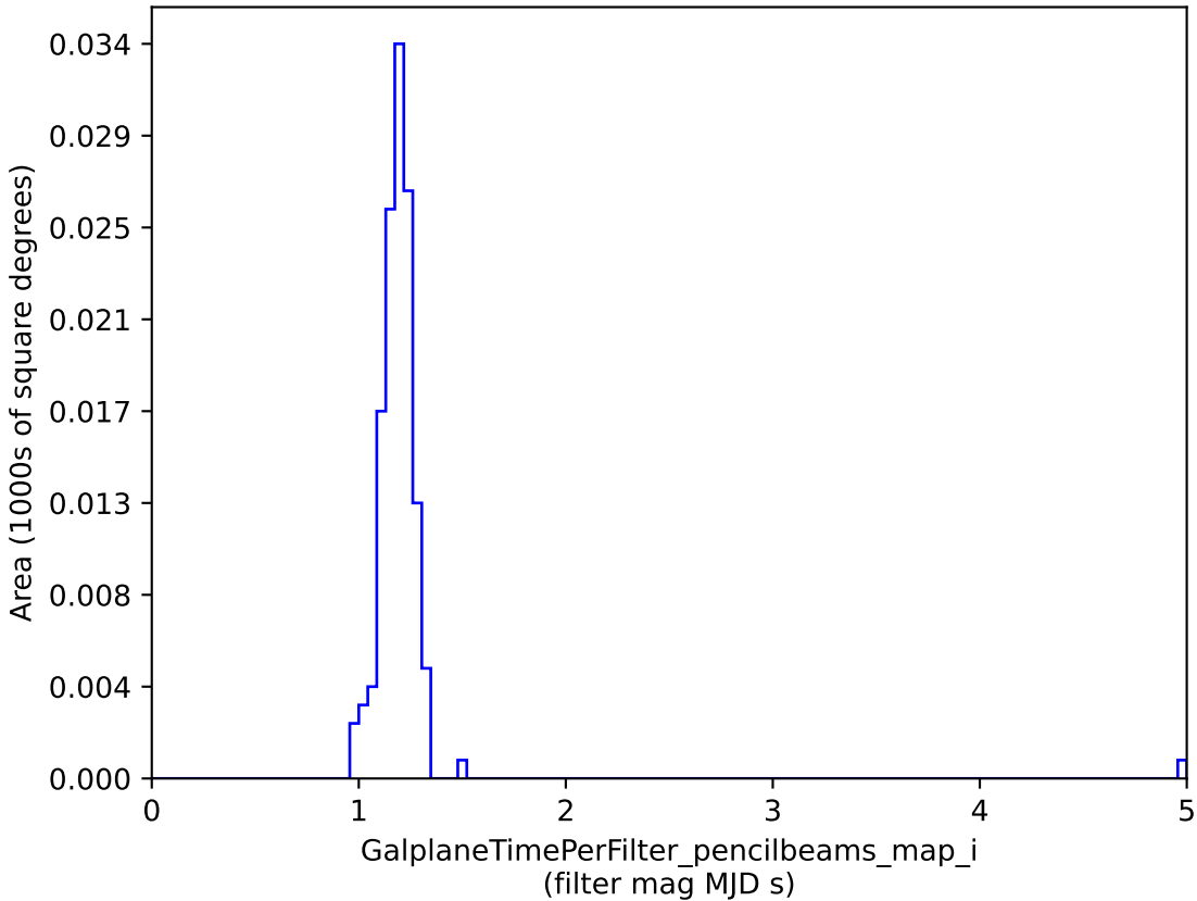
baseline_v3.2_10yrs : GalplaneTimePerFilter_pencilbeams_map_i
