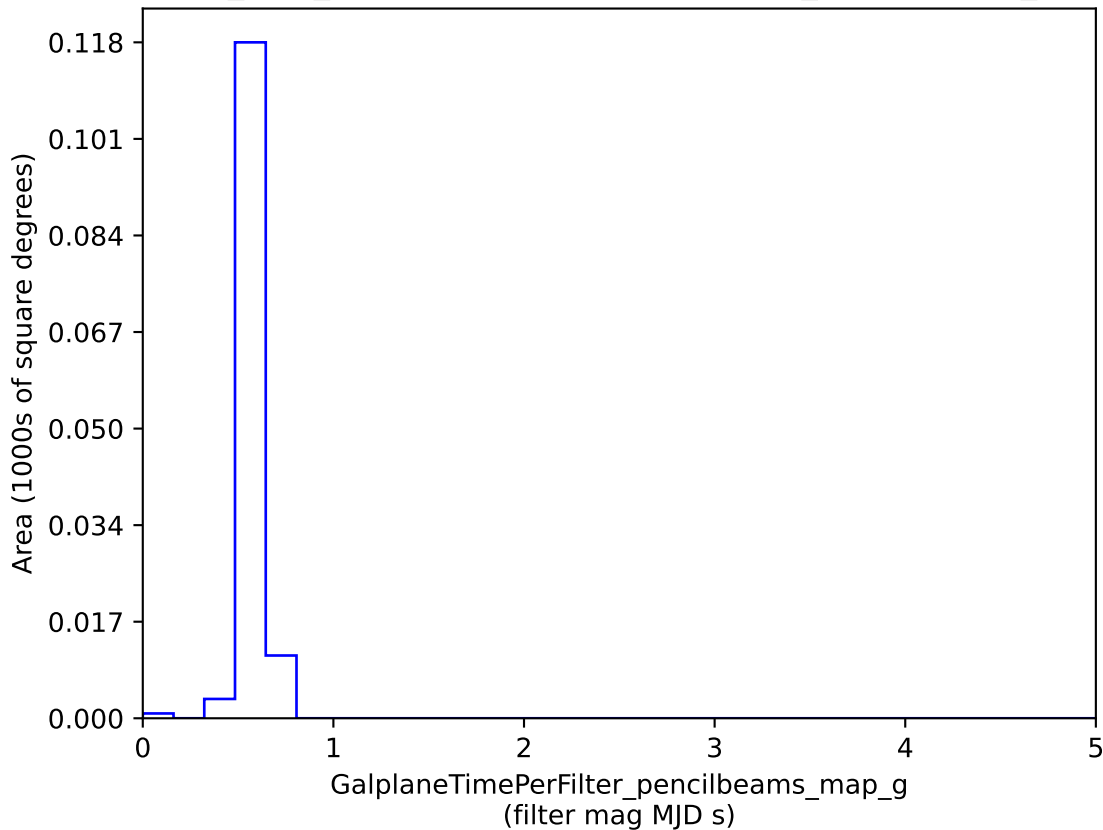
baseline_v3.2_10yrs : GalplaneTimePerFilter_pencilbeams_map_g
