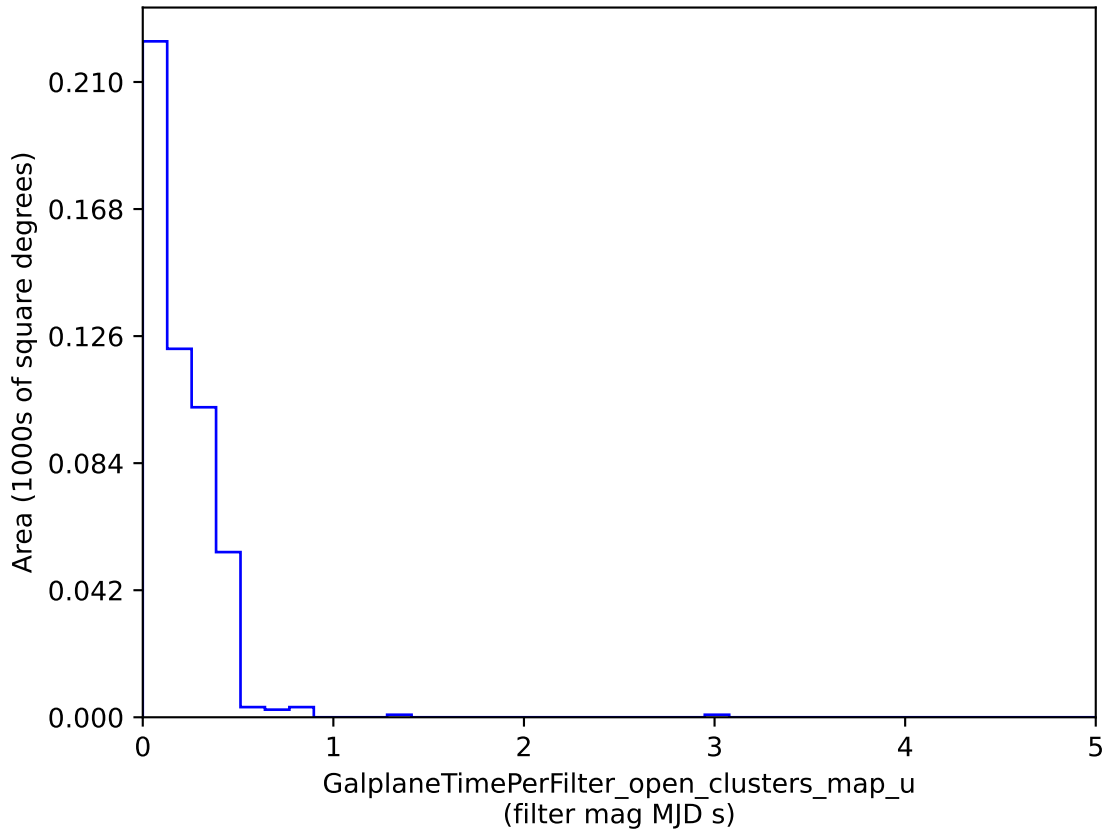
baseline_v3.2_10yrs : GalplaneTimePerFilter_open_clusters_map_u
