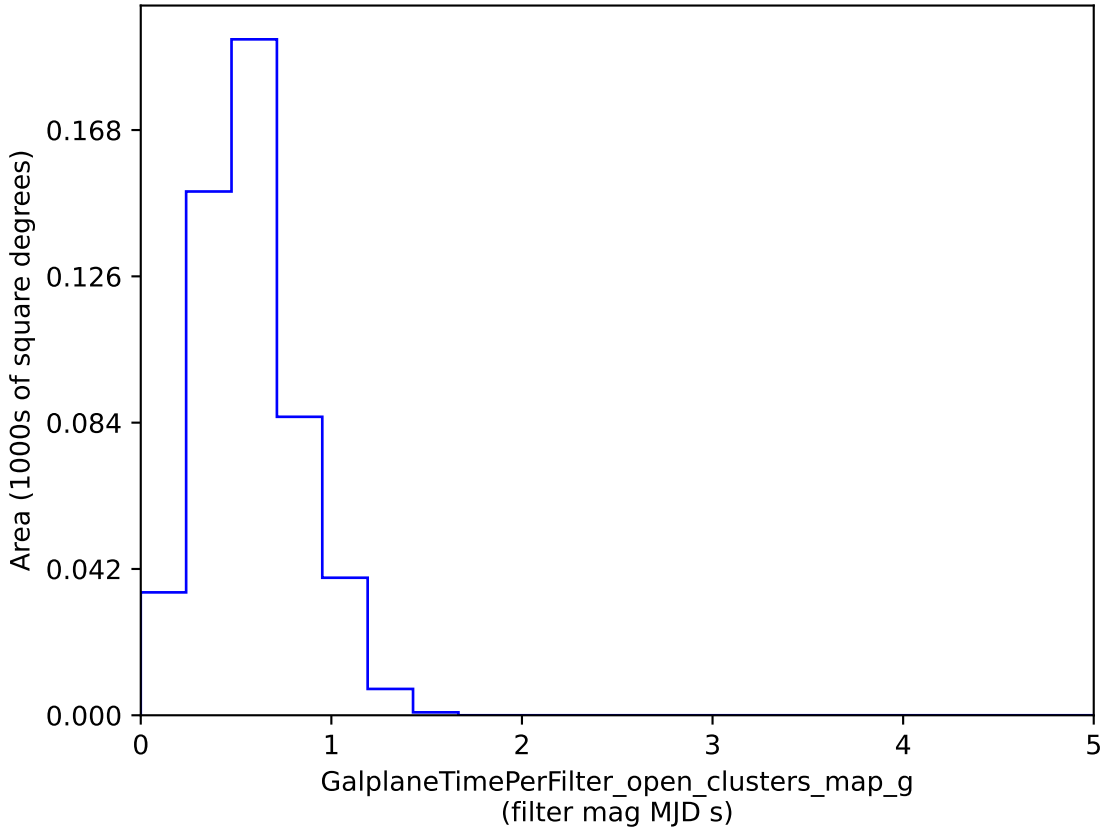
baseline_v3.2_10yrs : GalplaneTimePerFilter_open_clusters_map_g
