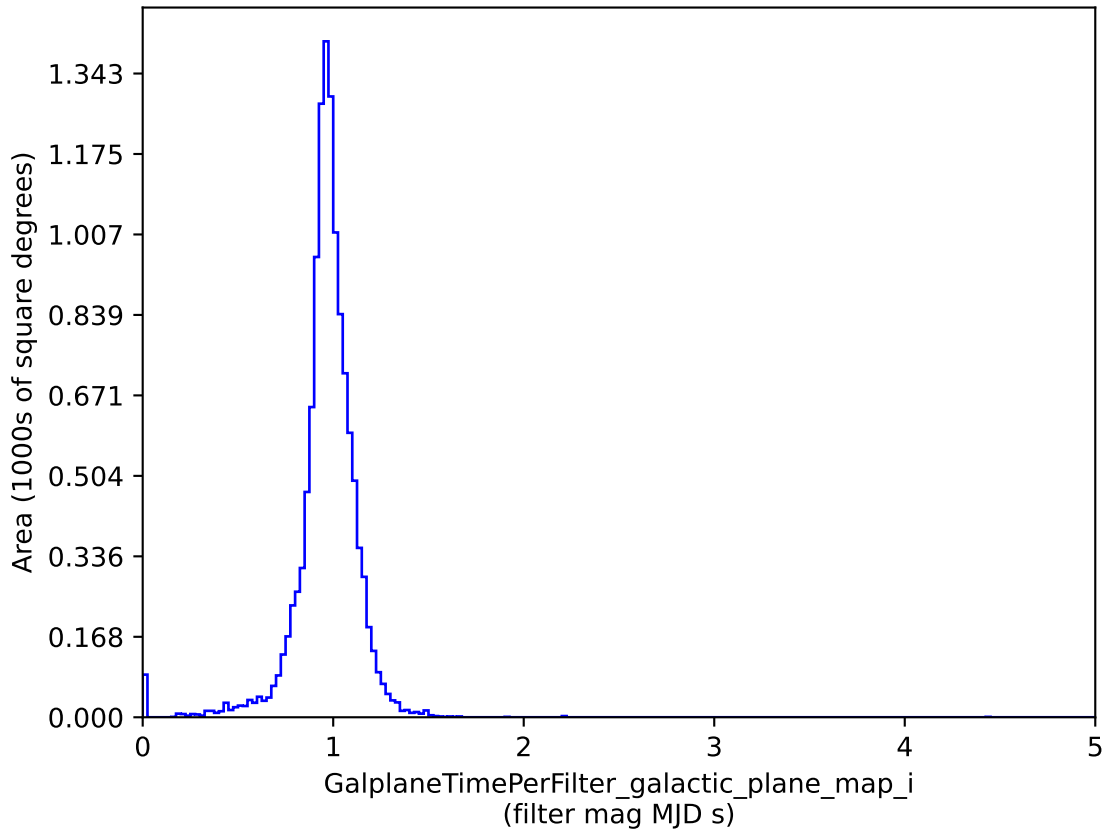
baseline_v3.2_10yrs : GalplaneTimePerFilter_galactic_plane_map_i
