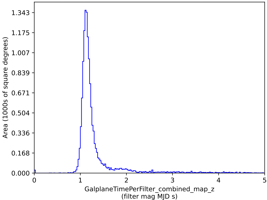
baseline_v3.2_10yrs : GalplaneTimePerFilter_combined_map_z
