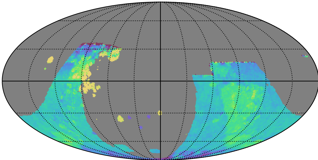
baseline_v3.2_10yrs : GalplaneTimePerFilter_combined_map_r
