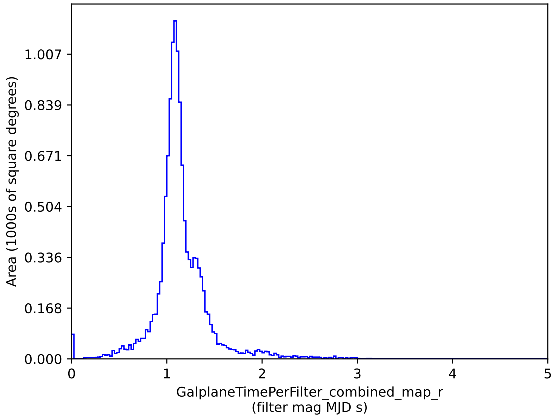
baseline_v3.2_10yrs : GalplaneTimePerFilter_combined_map_r
