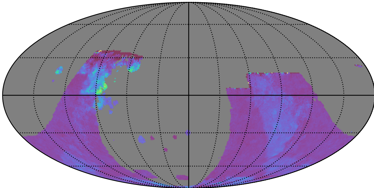
baseline_v3.2_10yrs : GalplaneTimePerFilter_combined_map_g
