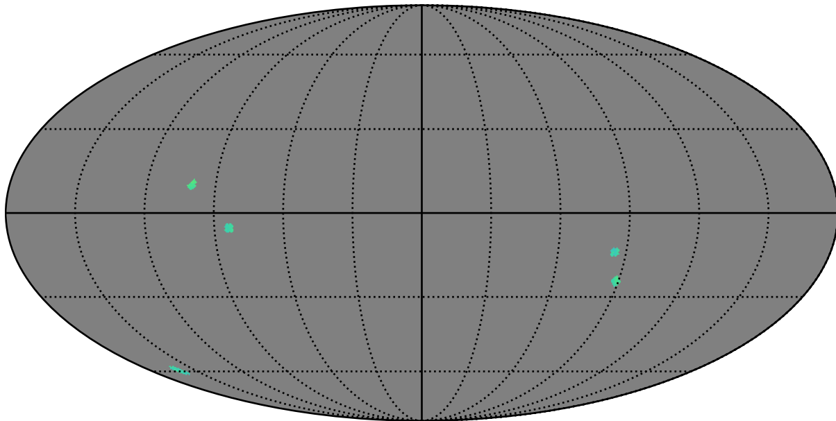
baseline_v3.2_10yrs : GalplaneTimePerFilter_bonito_sfr_map_z
