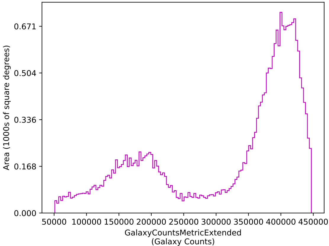
baseline_v3.2_10yrs z: GalaxyCountsMetricExtended
