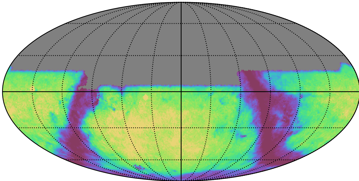
baseline_v3.2_10yrs u: GalaxyCountsMetricExtended
