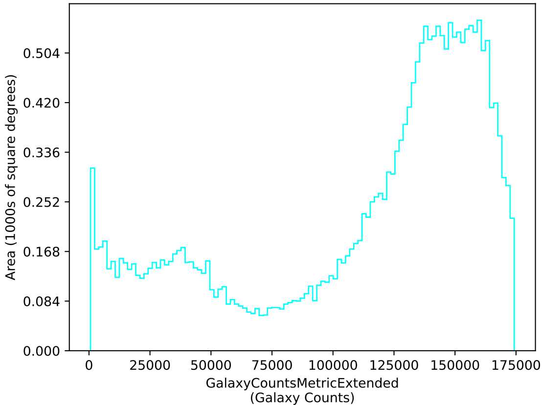
baseline_v3.2_10yrs u: GalaxyCountsMetricExtended
