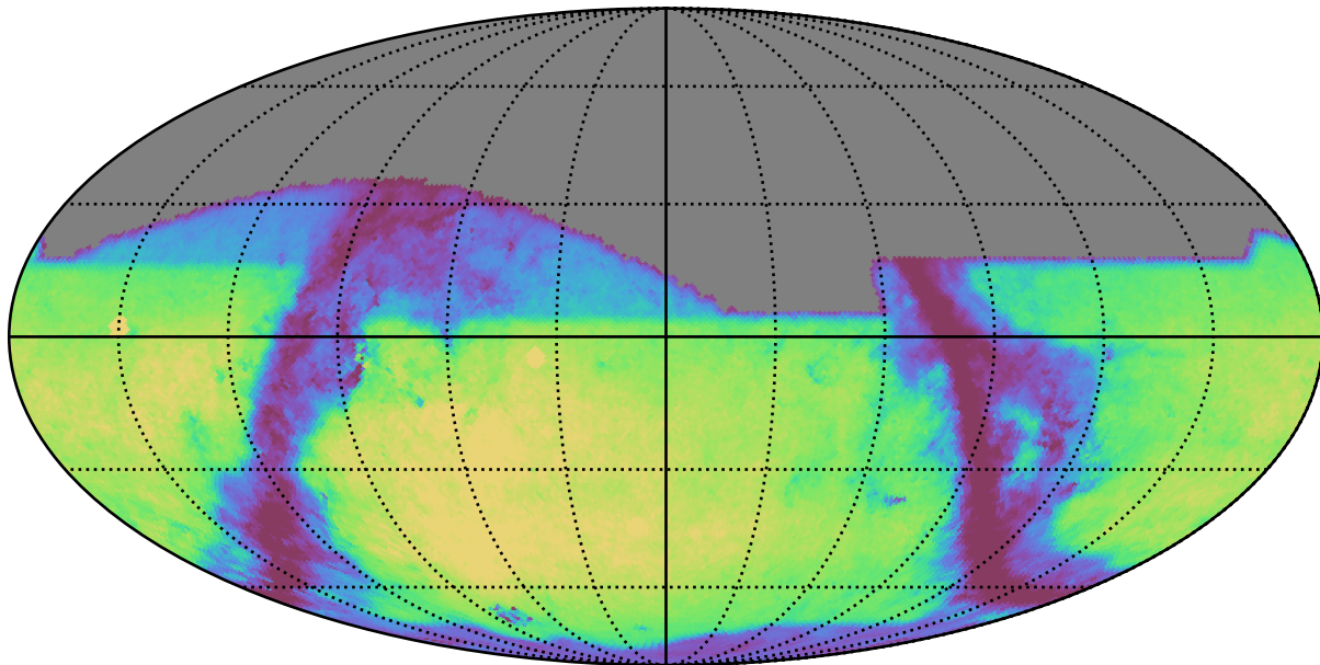
baseline_v3.2_10yrs r: GalaxyCountsMetricExtended
