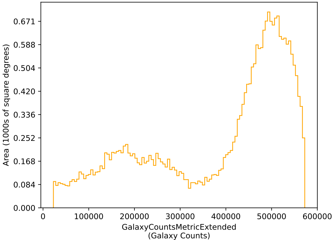
baseline_v3.2_10yrs r: GalaxyCountsMetricExtended
