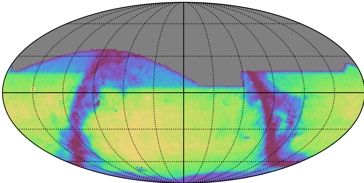
baseline_v3.2_10yrs i: GalaxyCountsMetricExtended
