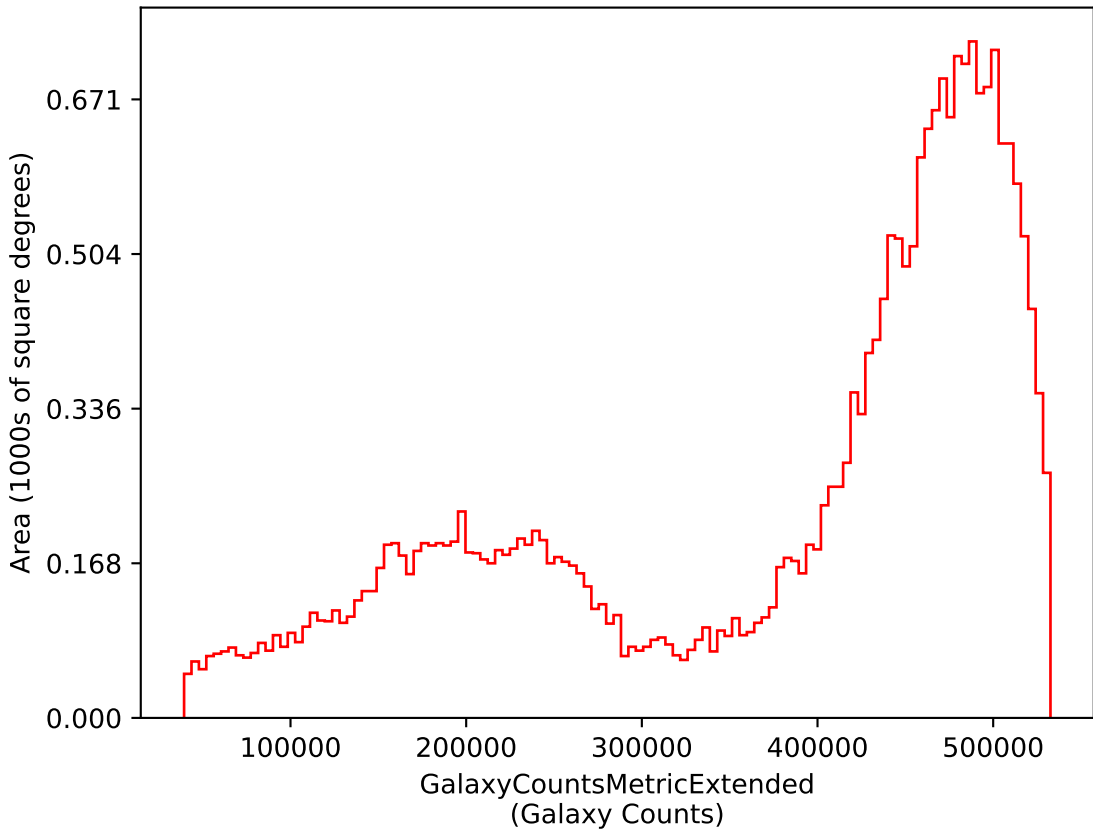
baseline_v3.2_10yrs i: GalaxyCountsMetricExtended
