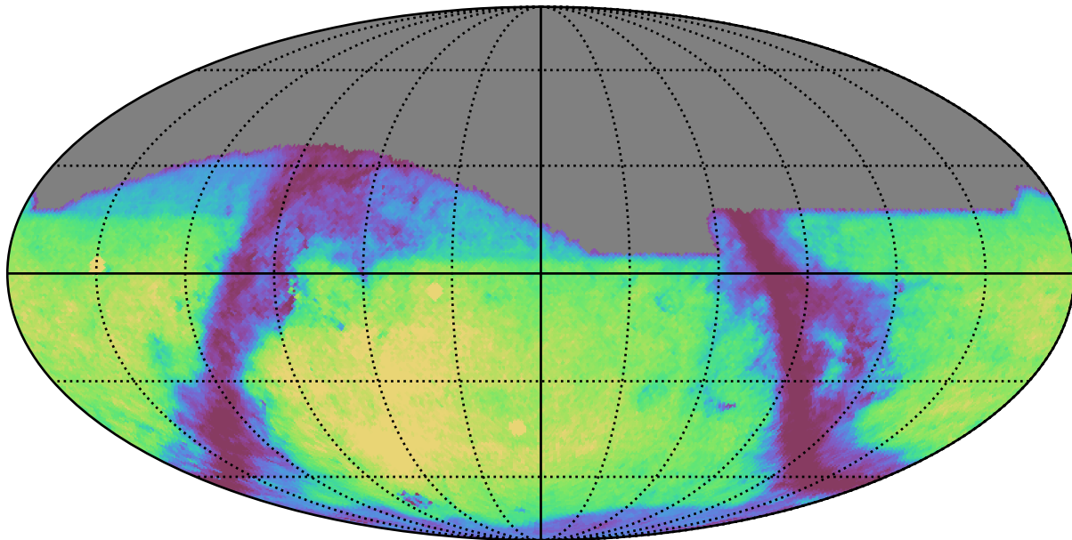
baseline_v3.2_10yrs g: GalaxyCountsMetricExtended
