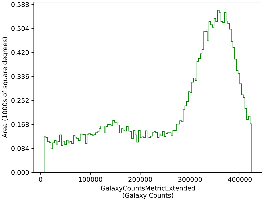
baseline_v3.2_10yrs g: GalaxyCountsMetricExtended
