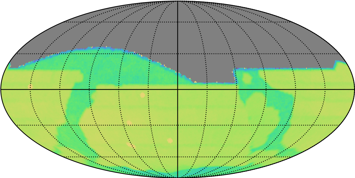
baseline_v3.2_10yrs : GalPlaneVisitIntervalsTimescales_xray_binaries_map_Tau_5_0
