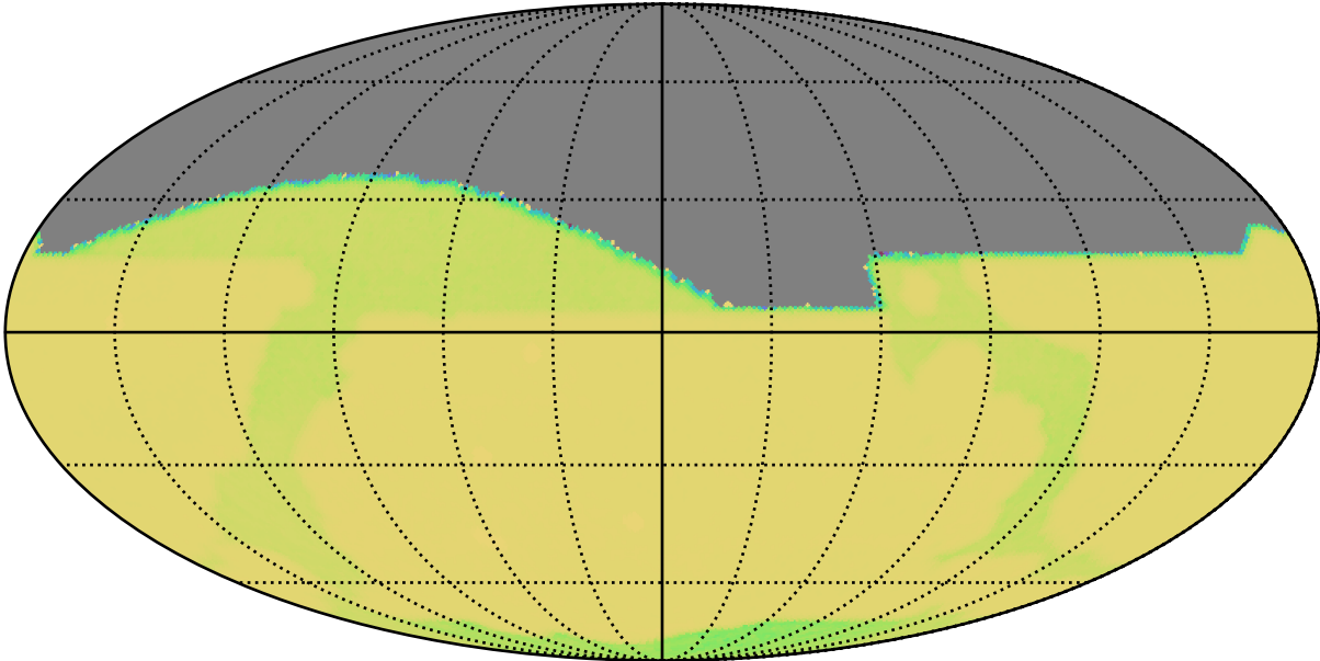
baseline_v3.2_10yrs : GalPlaneVisitIntervalsTimescales_xray_binaries_map_Tau_46_5
