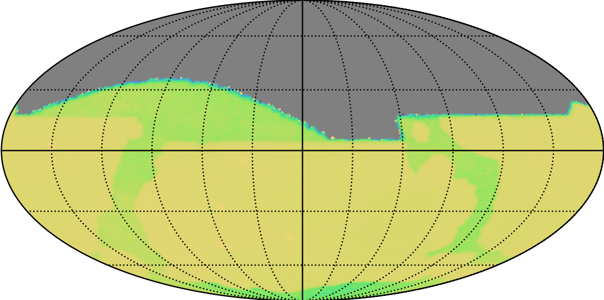
baseline_v3.2_10yrs : GalPlaneVisitIntervalsTimescales_xray_binaries_map_Tau_20_0
