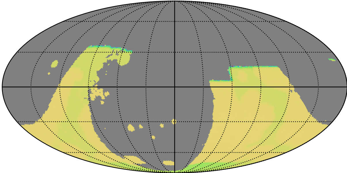
baseline_v3.2_10yrs : GalPlaneVisitIntervalsTimescales_combined_map_Tau_73_0
