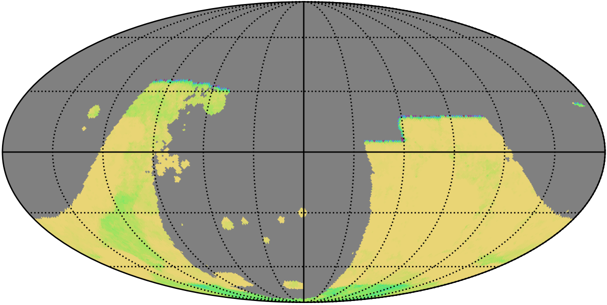
baseline_v3.2_10yrs : GalPlaneSeasonGapsTimescales_combined_map_Tau_232_5
