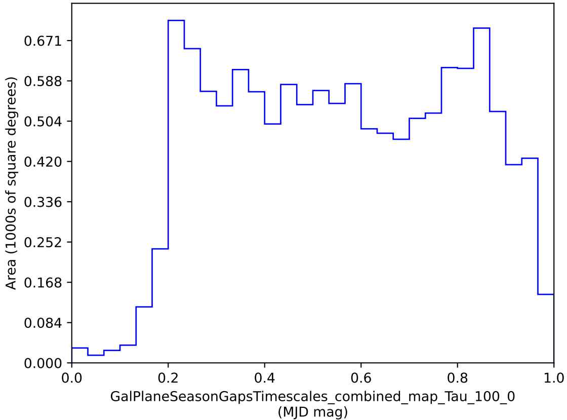
baseline_v3.2_10yrs : GalPlaneSeasonGapsTimescales_combined_map_Tau_100_0
