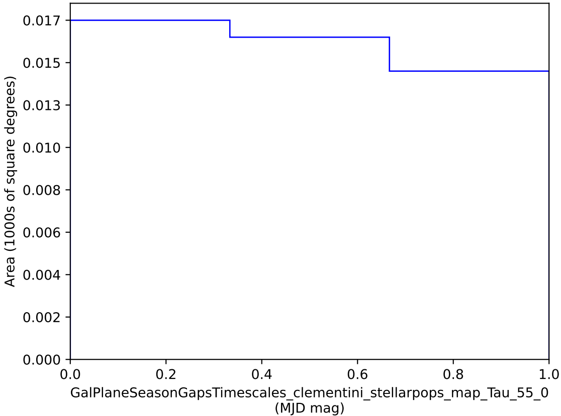
baseline_v3.2_10yrs : GalPlaneSeasonGapsTimescales_clementini_stellarpops_map_Tau_55_0
