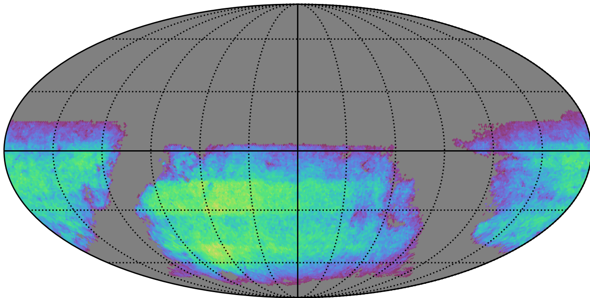
baseline_v3.2_10yrs i band non-DD year 9: ExgalM5WithCuts
