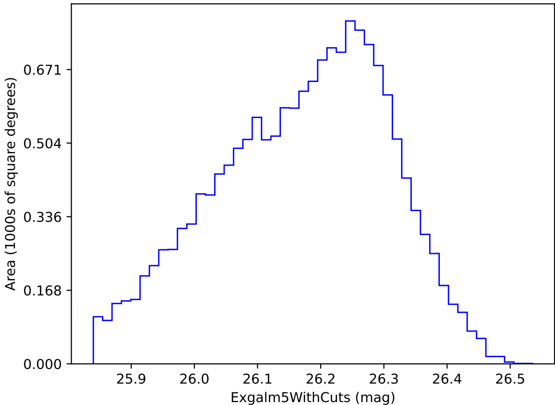
baseline_v3.2_10yrs i band non-DD year 9: ExgalM5WithCuts
