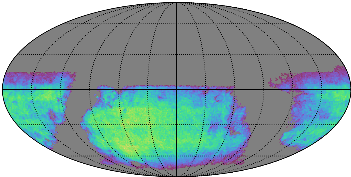
baseline_v3.2_10yrs i band non-DD year 8: ExgalM5WithCuts
