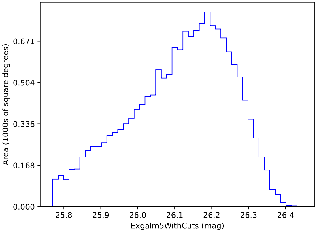
baseline_v3.2_10yrs i band non-DD year 8: ExgalM5WithCuts
