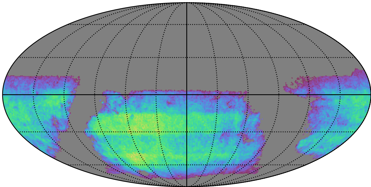
baseline_v3.2_10yrs i band non-DD year 7: ExgalM5WithCuts
