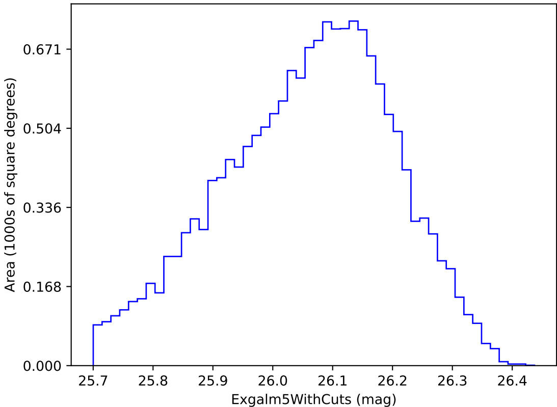
baseline_v3.2_10yrs i band non-DD year 7: ExgalM5WithCuts
