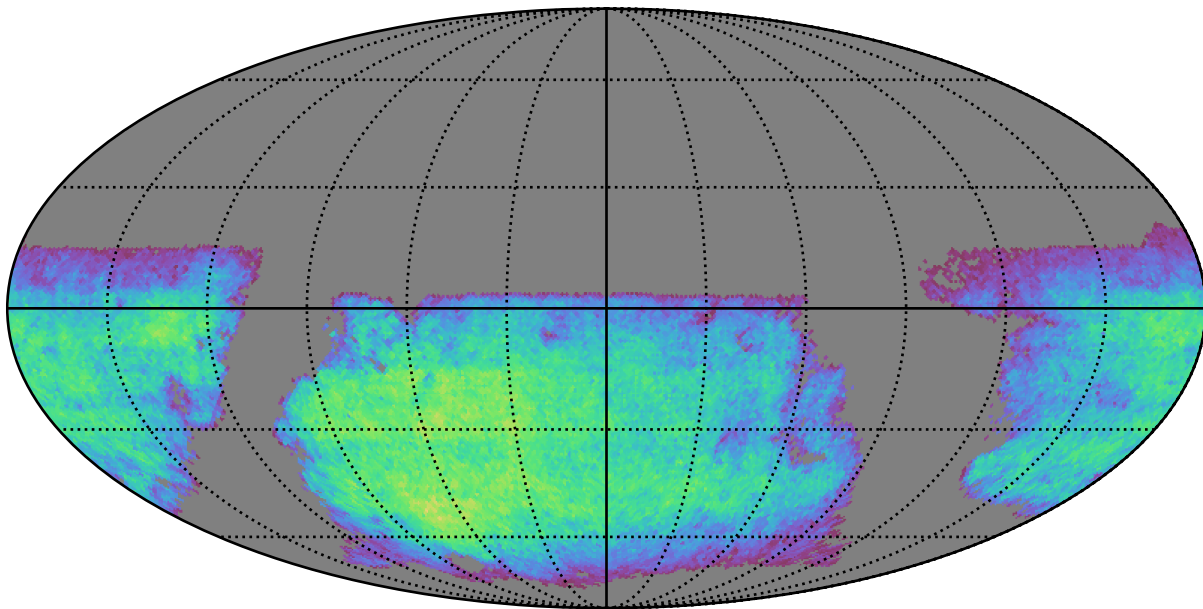
baseline_v3.2_10yrs i band non-DD year 6: Exgal m5 WithCuts
