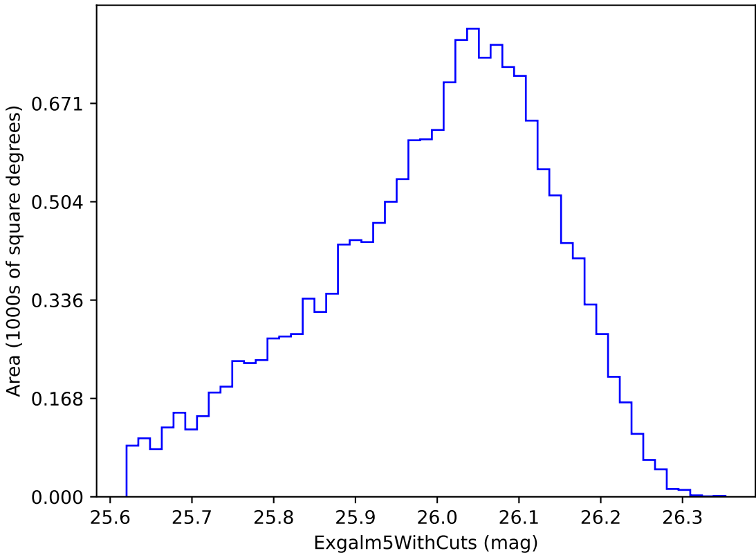
baseline_v3.2_10yrs i band non-DD year 6: ExgalM5WithCuts
