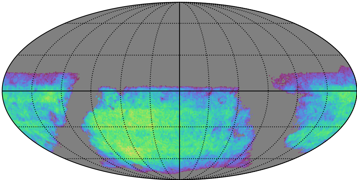
baseline_v3.2_10yrs i band non-DD year 4: ExgalM5WithCuts
