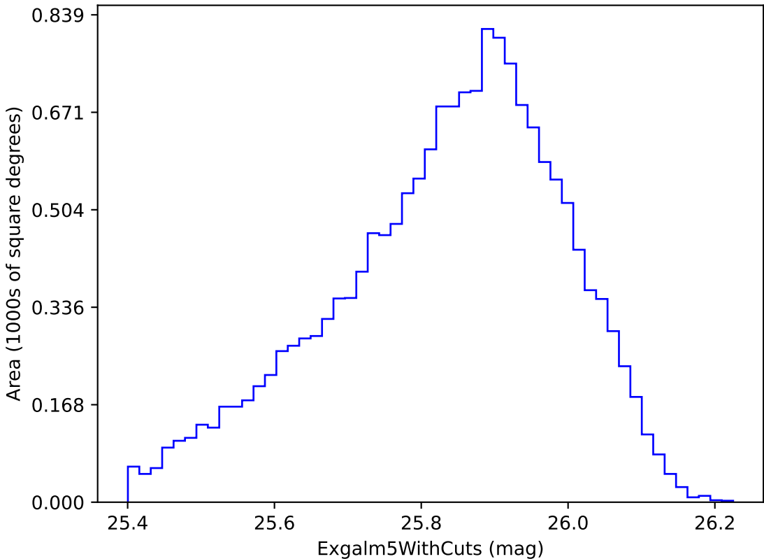
baseline_v3.2_10yrs i band non-DD year 4: ExgalM5WithCuts
