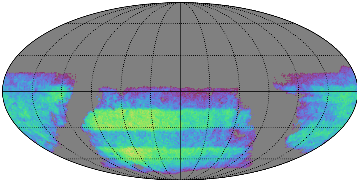
baseline_v3.2_10yrs i band non-DD year 3: ExgalM5WithCuts
