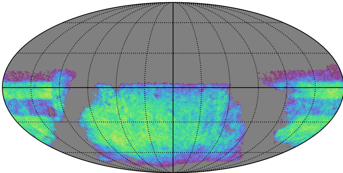
baseline_v3.2_10yrs i band non-DD year 2: ExgalM5WithCuts
