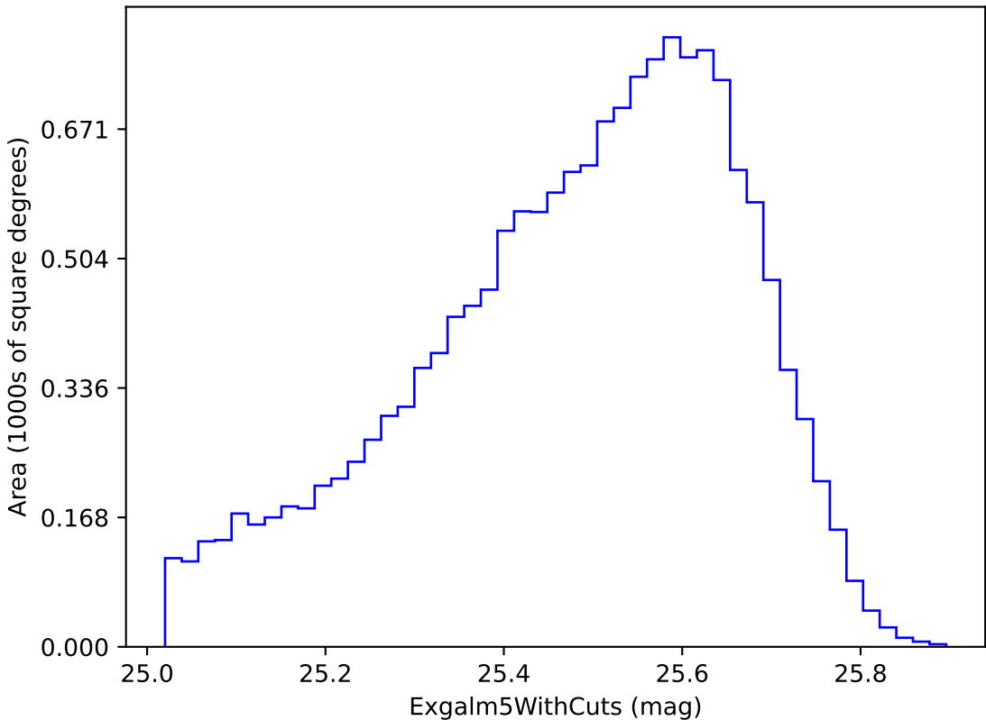
baseline_v3.2_10yrs i band non-DD year 2: ExgalM5WithCuts
