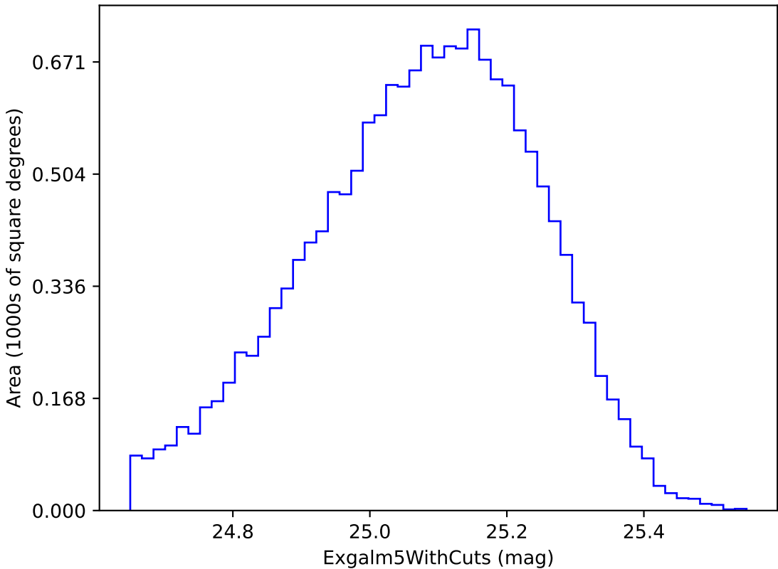
baseline_v3.2_10yrs i band non-DD year 1: ExgalM5WithCuts
