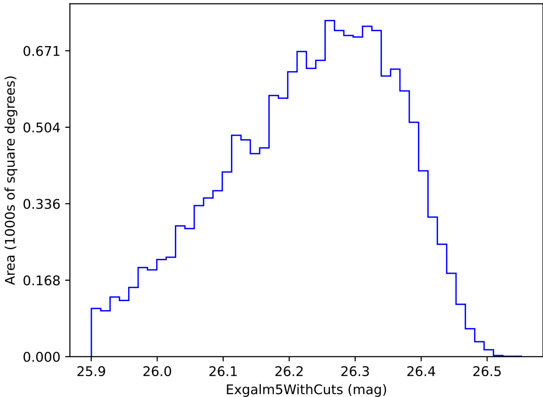
baseline_v3.2_10yrs i band non-DD year 10: ExgalM5WithCuts
