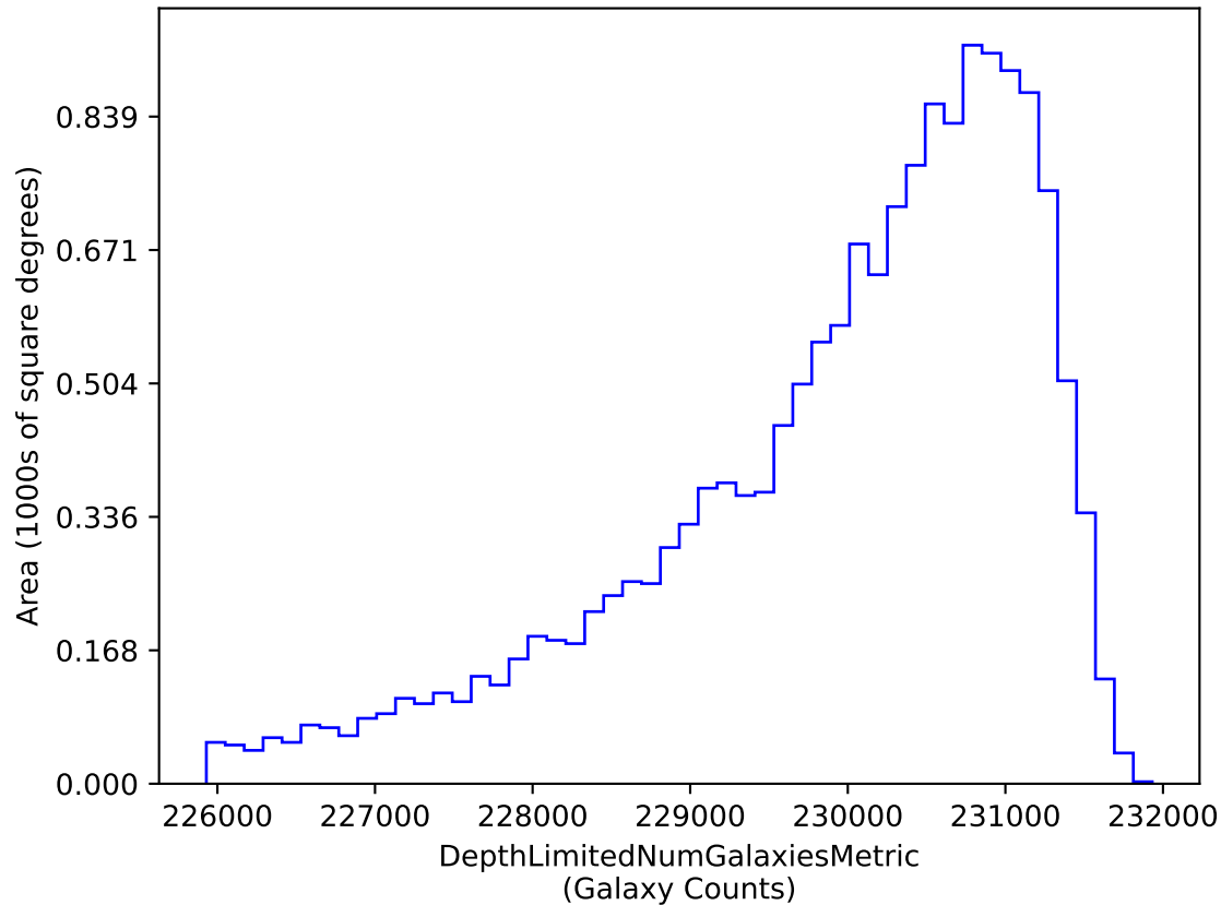
baseline_v3.2_10yrs i band galaxies non-DD: DepthLimitedNumGalaxiesMetric
