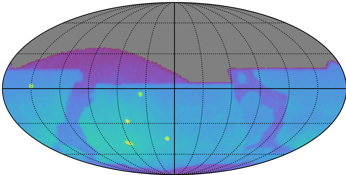
baseline_v3.2_10yrs : Brown Dwarf, L7
