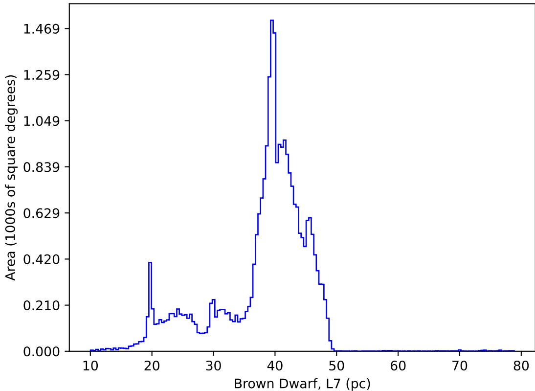
baseline_v3.2_10yrs : Brown Dwarf, L7
